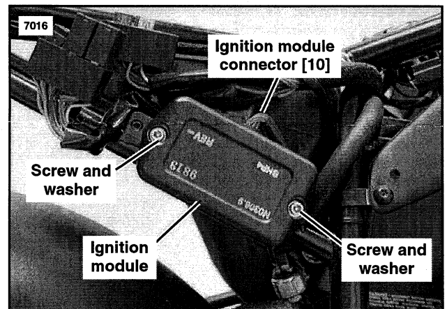
Figure 3. Ignition Module
